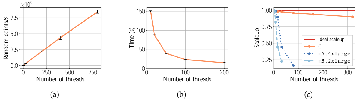
Figure 3: (a) Scalability of a Monte Carlo simulation to approximate \rho . CRUCIAL reaches 8.4 billion random points per second with 800 threads. (b) Scalability of a Mandelbrot computation with CRUCIAL. (c) Scalability of the k -means clustering algorithm with VM threads versus FaaS with CRUCIAL.
